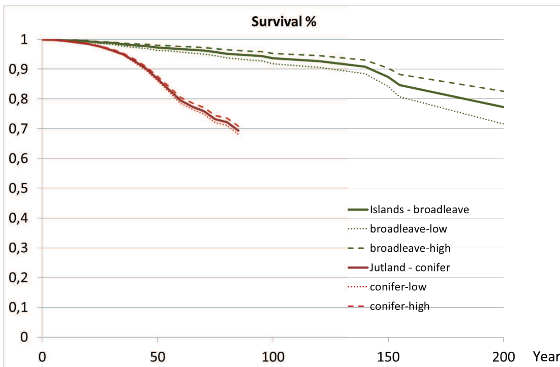
Figure 22 Predicted survival probabilities and their uncertainties as result of growth region, tree species and age classes.
