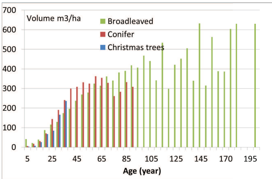
Figure 20 Growing stock (above-ground biomass \text{m}^3 \text{ha}^{-1} ) by age class distribution by 2010, for broadleaved, conifers and Christmas trees.
